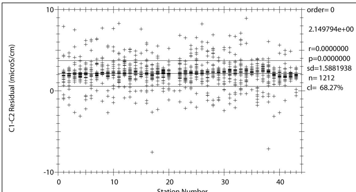
Figure 3. Uncorrected C1 and C2 conductivity differences by cast (-0.005°C ≤ T1-T2 ≤ 0.005°C).
