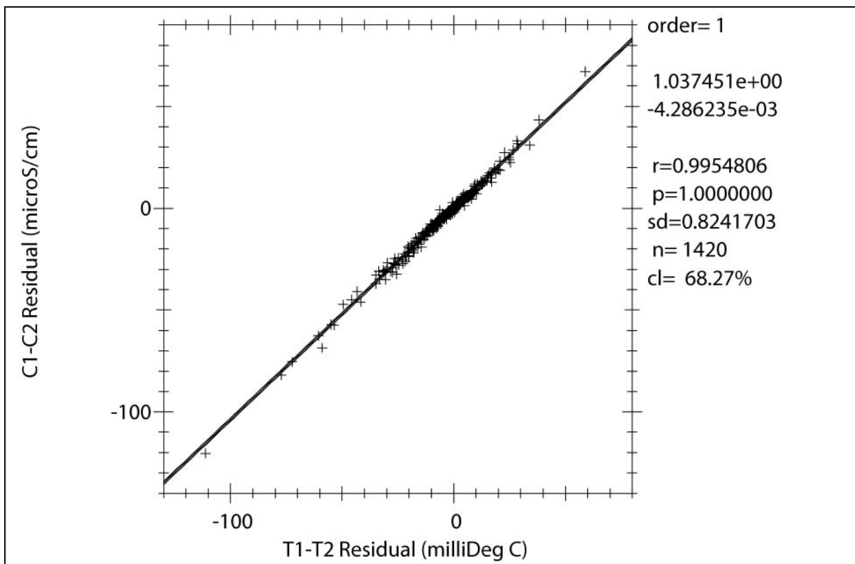
Figure 2. C1-C2 by T1-T2, all points.
